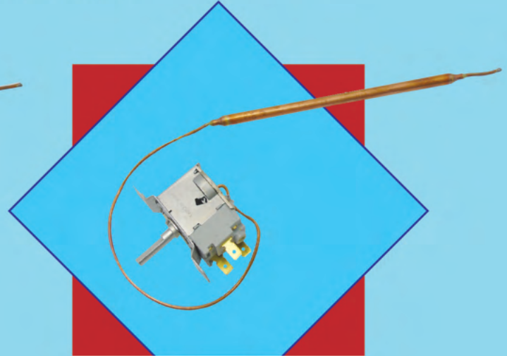
ARAH-THCH-68 THERMOSTAT ZAMIL H/C CHINA
