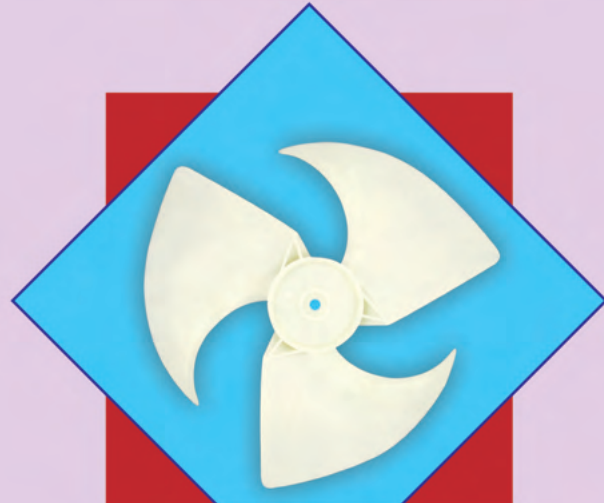
ARAH-SFSR-004 REPLACEMENT FOR SPLIT A/C FAN BLADE SAMSUNG RIGHT(DIA 37.5 x H11.3 cm)
