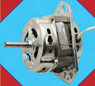
ARAH-WMWM - 178 WM WASH MOTOR 200W 12 MM
